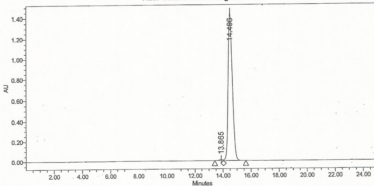
Auto-Scaled Chromatogram
